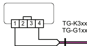
Figure 4: Wiring of floor or duct sensor when using internal setpoint
