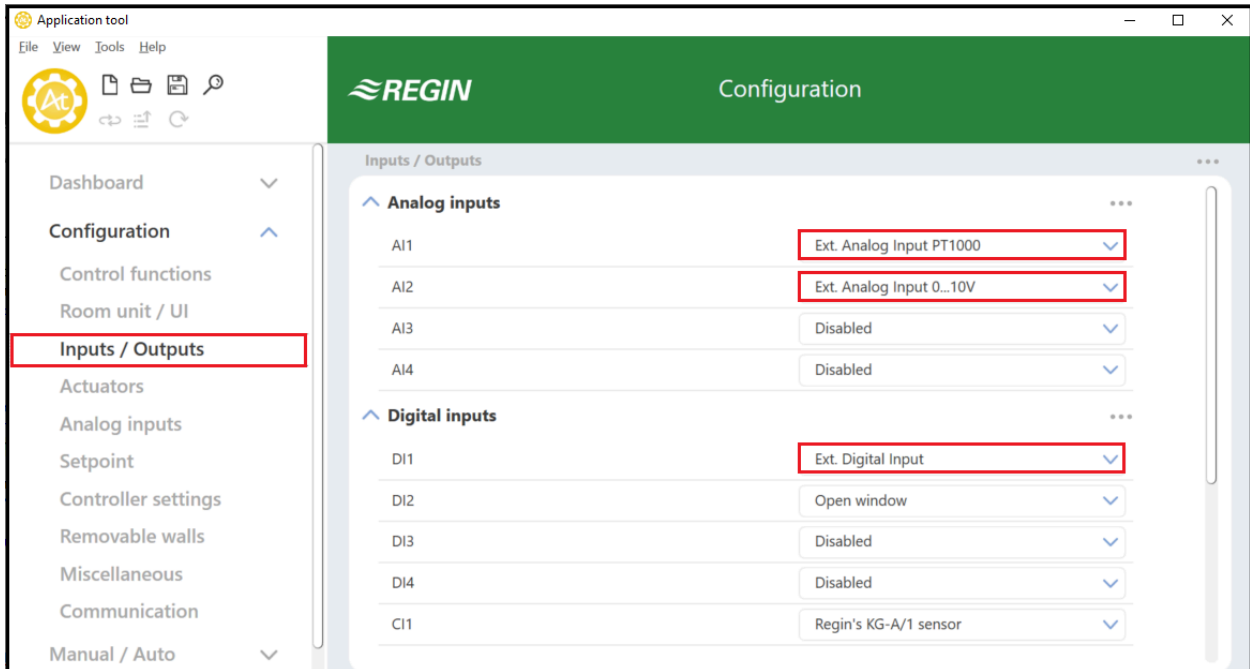
Figure 4-2 Controller input configuration in Application tool
