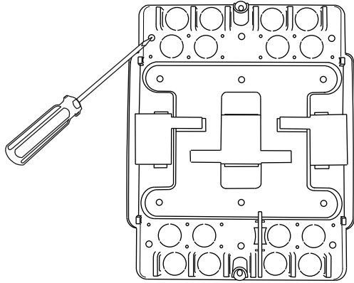
Figure 8-2 Attaching the baseplate to the wall.
