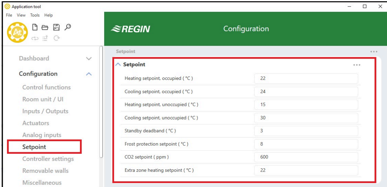
Figure 5-1 Setpoint and deadband configuration settings in Application tool.
