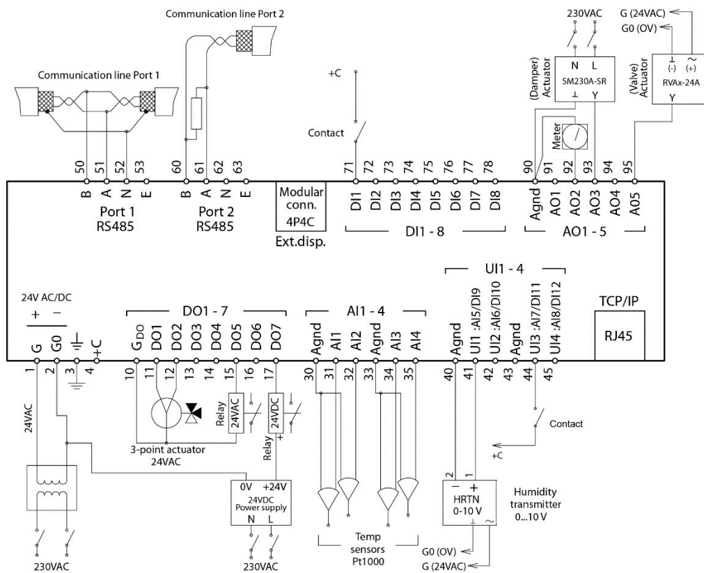
Figure 4-3 Wiring example
