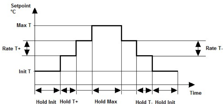
Figure 3-9 Screed drying
