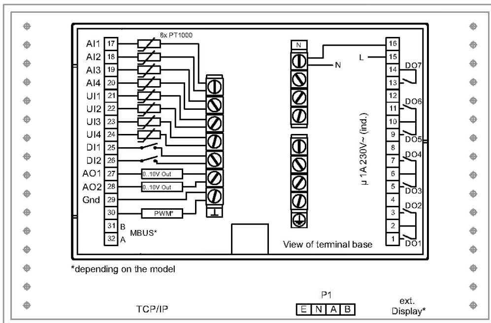
Figure 4-2 Terminal positions 230 V models (Exigo Vido)
