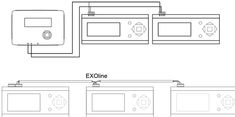
Figure 4-1 | Expansion units EXOline
