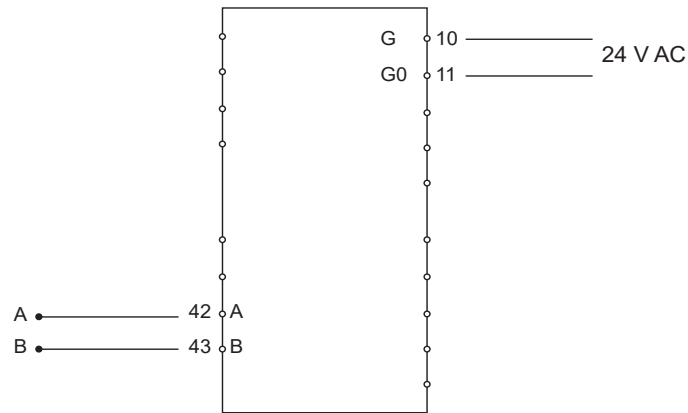
Figure 1 Wiring
