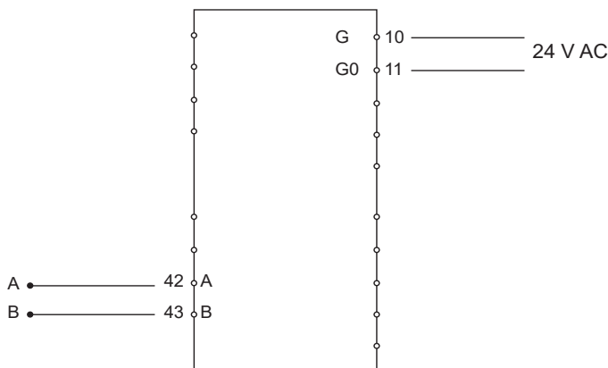
Figure 1 Wiring
