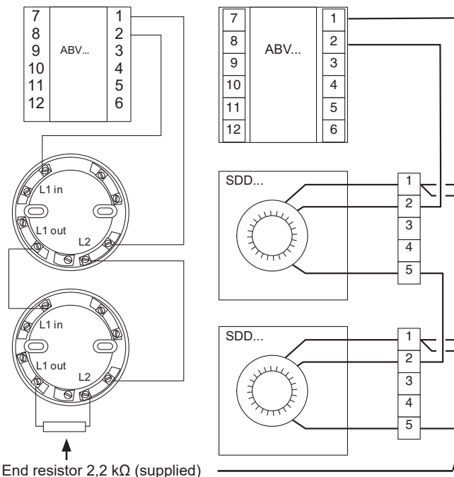
Wiring ABV(24)S-300/D and S65...
