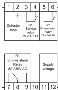
Wiring ABV(24)S-300/D
