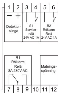
Figur 1. Inkoppling ABV(24)-S-300/D
