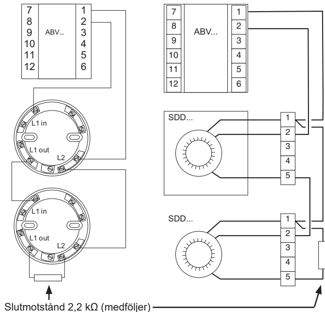
Figur 2. Inkoppling ABV(24)-S-300/D och S65... Inkoppling ABV(24)-S-300/D and SDD...
