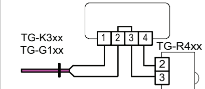
Figure 5: Wiring of an external, separate sensor and TG-R4xx as a setpoint device only
