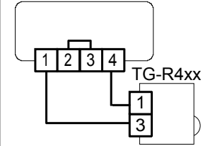
Figure 3: Wiring of TG-R430 sensor as external sensor and setpoint adjustment for room control
