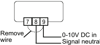
Figure 8 Wiring of external control signal
