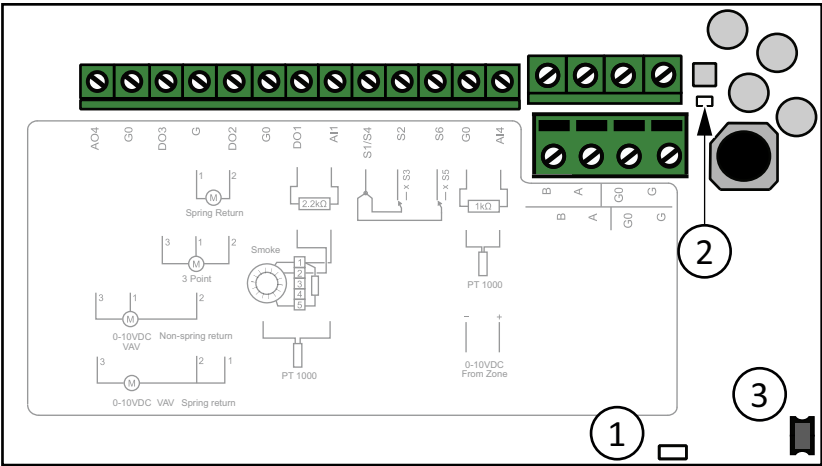
Figur 2-4 Inuti SCS-S2
