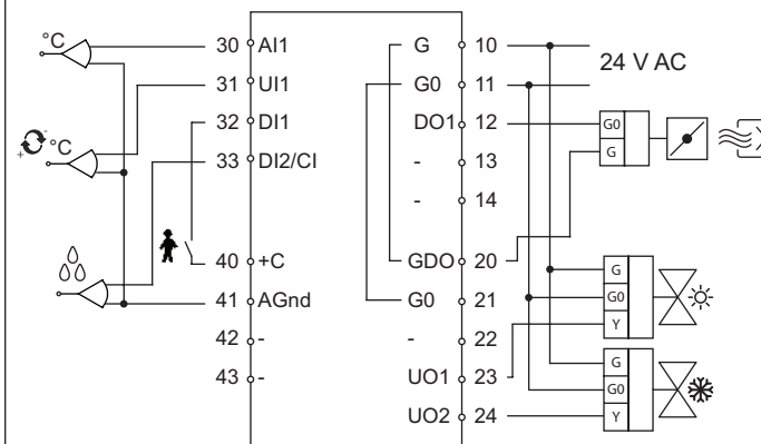
Figure 4. Connection diagram for RC
