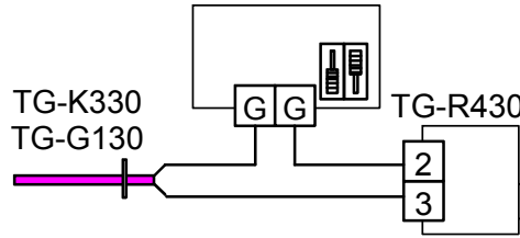
Figure 5: Switch setting and wiring for room control using external separate sensor and TG-R430 as setpoint
