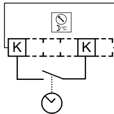
Figure 7: Wiring of the night set-back function
