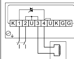
Figure 1 Wiring of supply voltage and output load, with screw terminal to connect earth and bypass to connected heat load.
