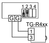
Figure 4 Switch setting and wiring for room control using TG-R4xx as sensor and setpoint.
