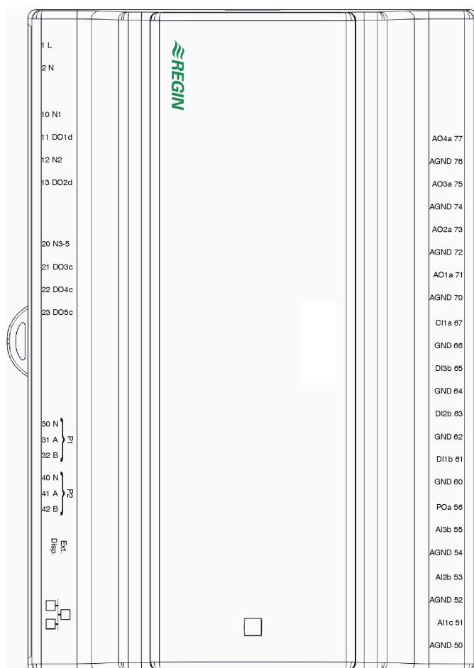
Figure 4-1 XCE163W-1 controller terminals layout
