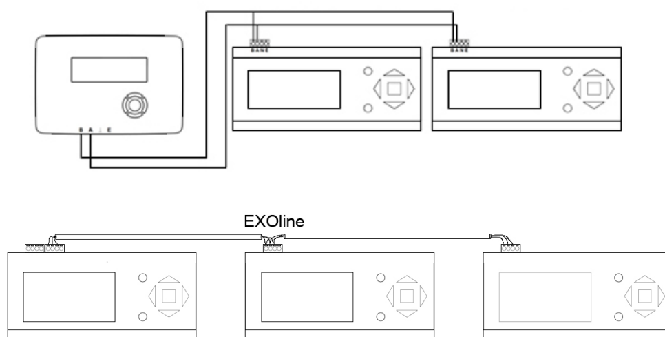
Figur 4-11 Expansionsenheter EXOline
