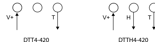
Figure 1 V+ = 11 + (0.02 \times RL) \dots 30 V DC, H and T = 4...20 mA
