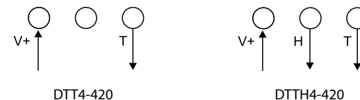
Fig. 1 | V+ = 11 + (0,02 \times RL) \dots 30 V DC, H et T = 4...20 mA
